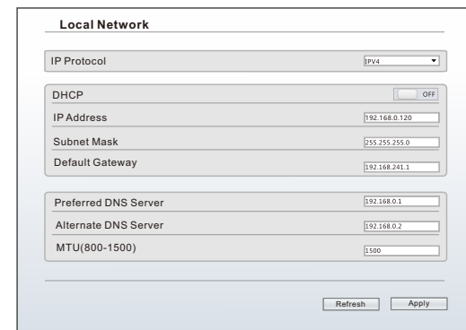
Figure 3-2 Local Network
